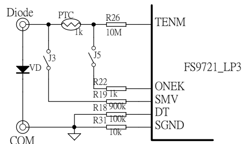
Diagram 29 Diode Measurement
