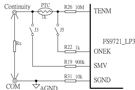
Diagram 30 Open-Short Tests
